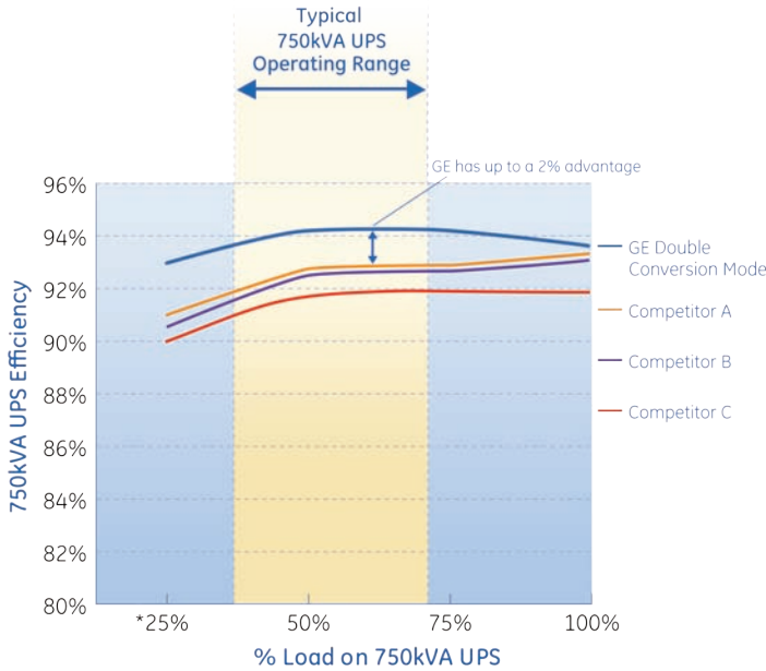
SG 750 kVA UPS Efficiency
